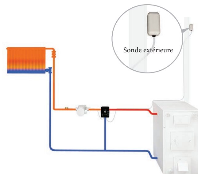
LK 110 SMARTCOMFORT
